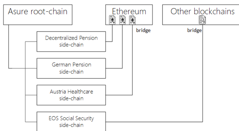
Figure 2: Asure side-chains
